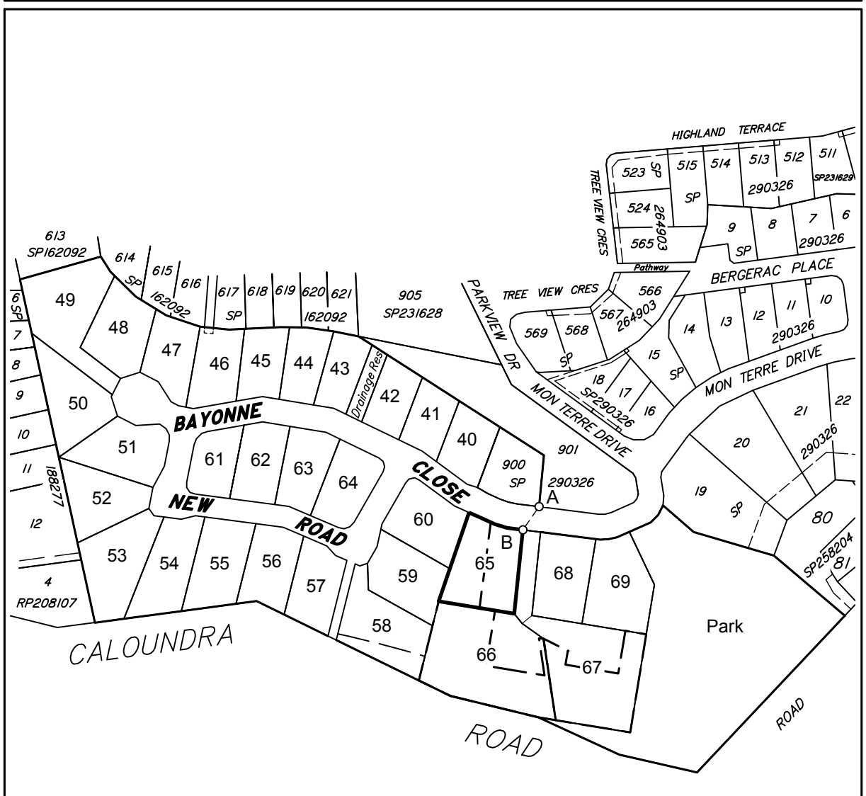
Cadastral Connection A-B 215°02' 15.83
